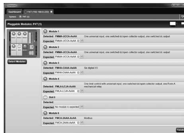
Pluggable modules view simplifies configuration by showing hardware present.
